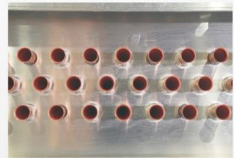
Expanded ends of Tubes
